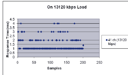
Figure.5: 13120 Kbps response times
