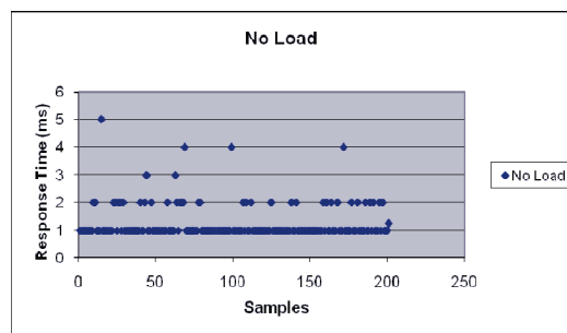
Figure.4: No load response times
