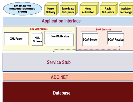
Figure.2: Architecture of the interoperability framework
