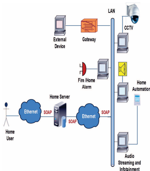
Figure.3: System implementation of interoperability framework
